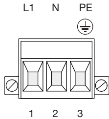
Rastermaß = 7,62mm
